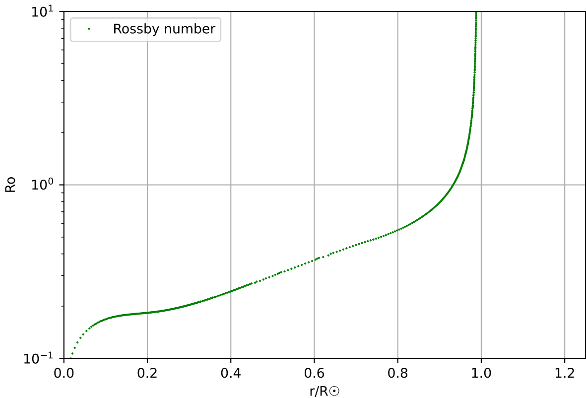
Rossby number, profile 146, age 4.44 \times 10^9
